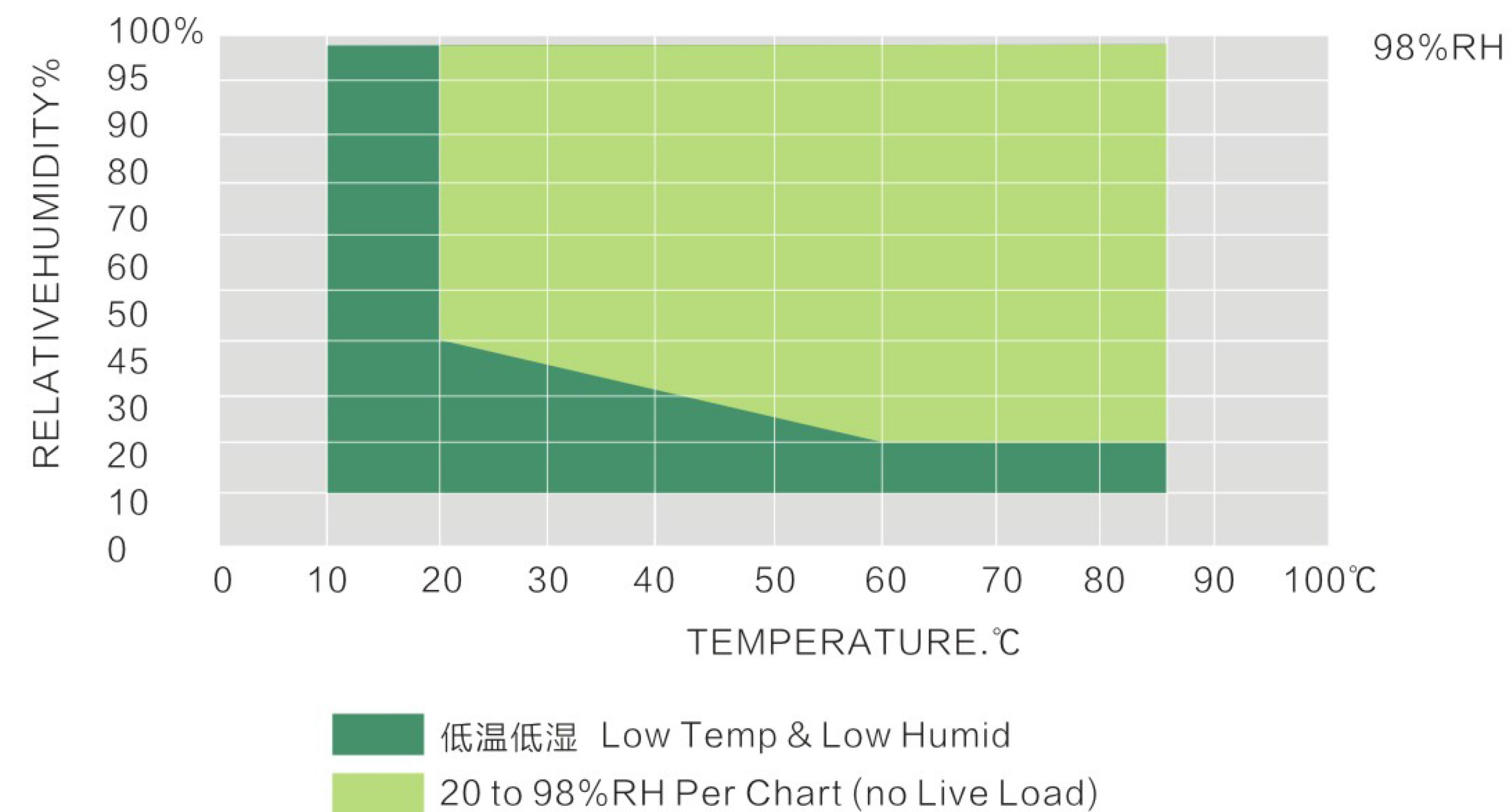
温湿度对照表 Temperature And Humidity Chart
